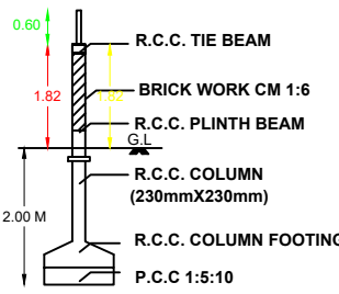
COMPOUND WALL DETAILS
