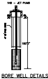
BORE WELL DETAILS
