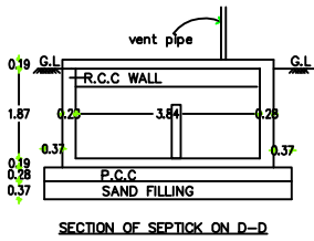
SECTION OF SEPTIC ON D-D
