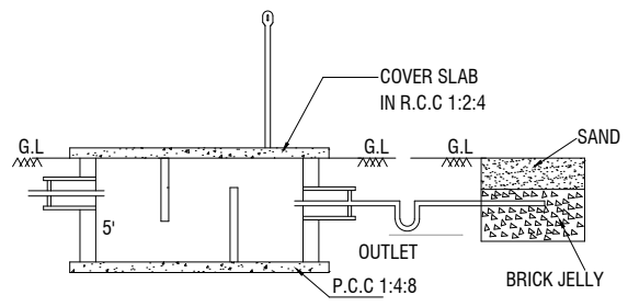
SECTION-AB
