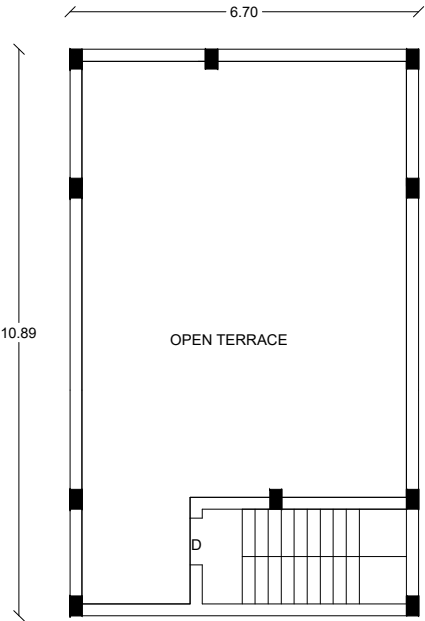
TERRACE FLOOR
