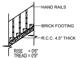
SECTION
