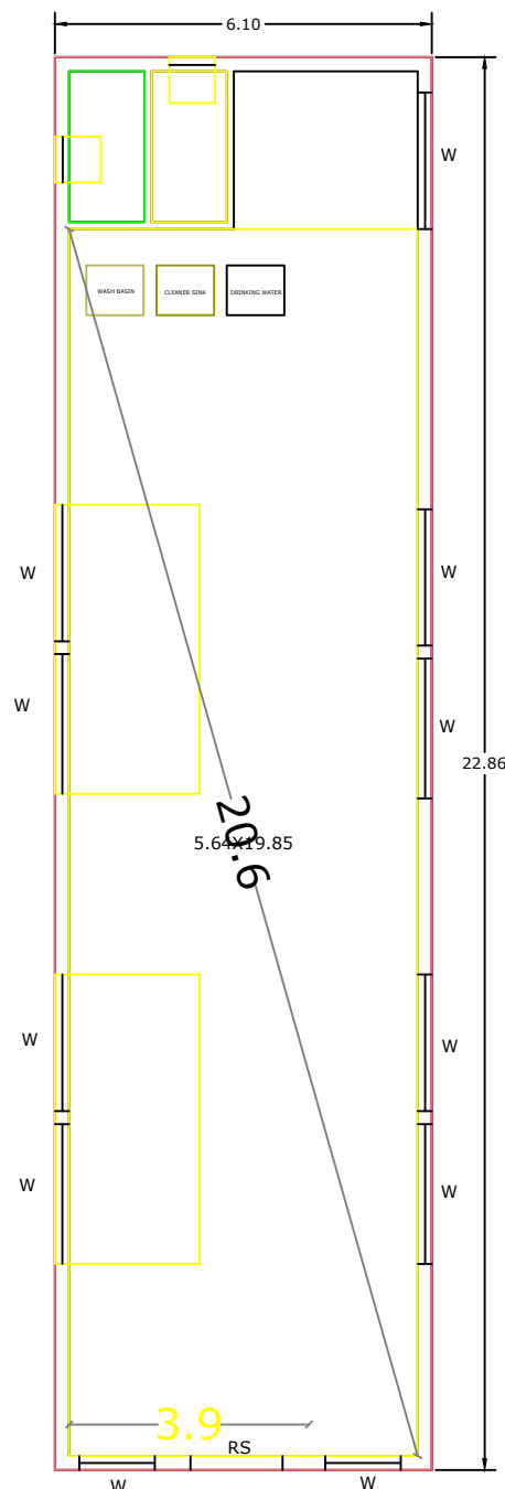
PRO GROUND FLOOR PLAN
