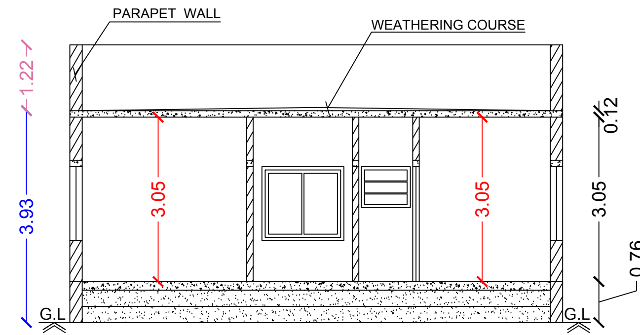
Section on-"AA"
