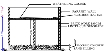
Section on-"AA"
