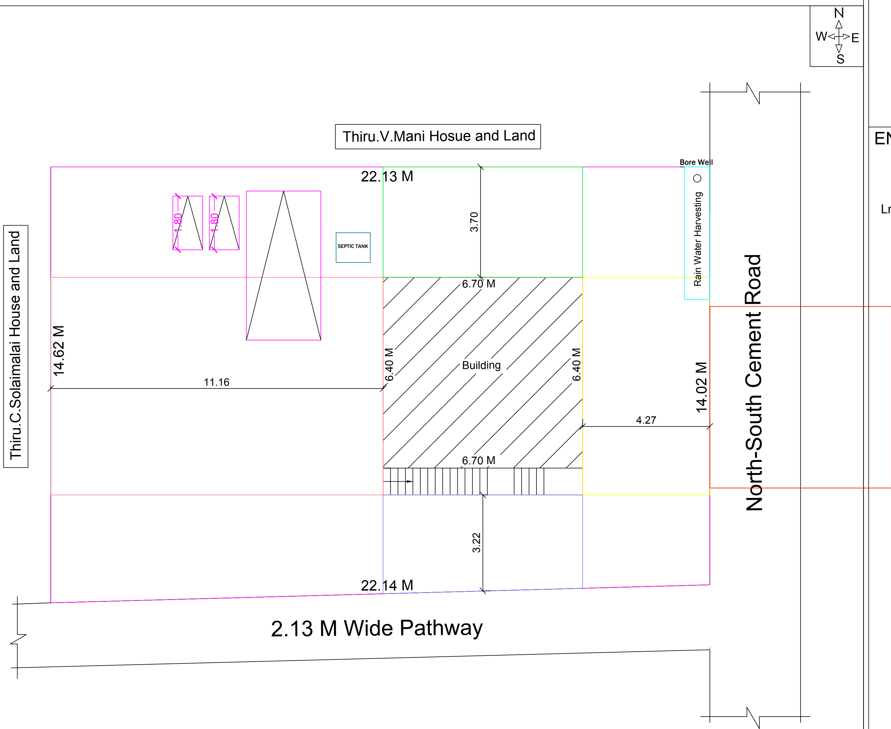
PLAN SEPTIC. TANK
