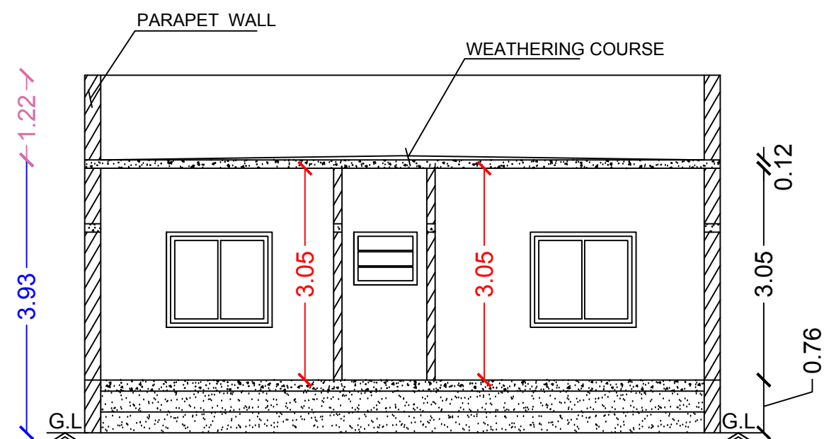
Section on-"AA"
