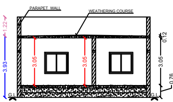
Section on-"AA"
