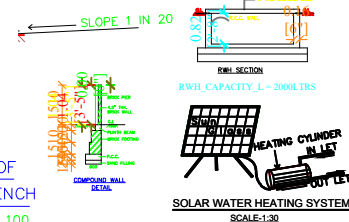
SOLAR WATER HEATING SYSTEM SCALE: 1:30
