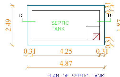
SEPTIC TANK
