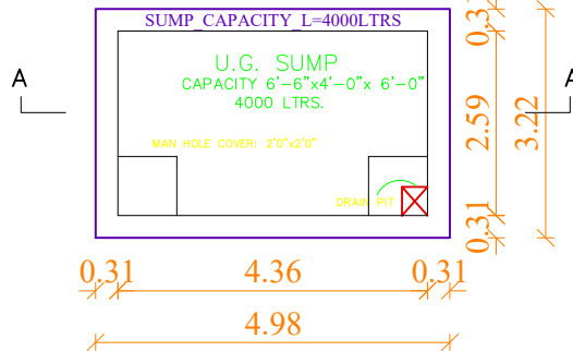
SUMP DETAIL
