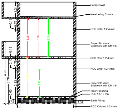
SECTION ON "VR"
