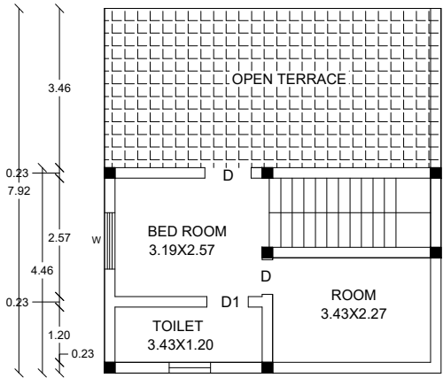
EXT & PRO FIRST FLOOR
