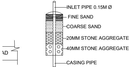
DETAILS OF RAIN WATER HARVESTING STRUCTURES
