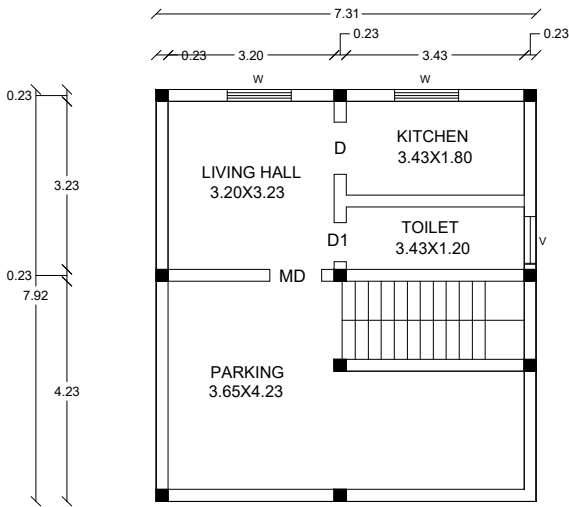
EXT GROUND FLOOR
