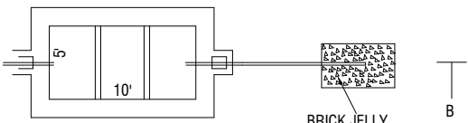
SEPTIC TANK & DISPERSION TRENCH DETAILS
