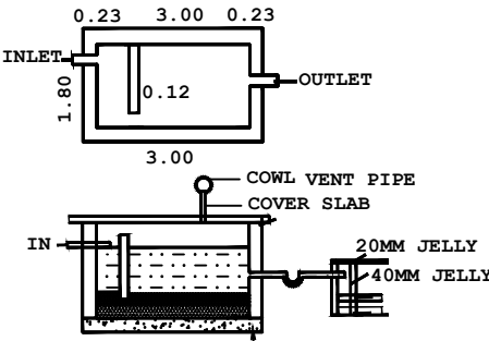
SEPTIC TANK NOT TO SCALE
