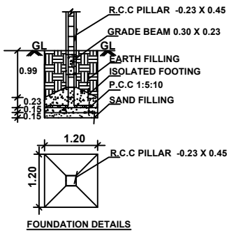
FOUNDATION DETAILS
