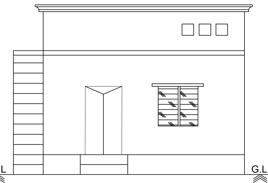
FRONT ELEVATION
