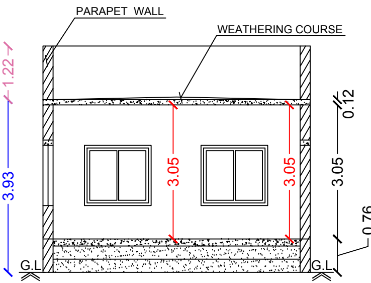
Section on-"AA"
