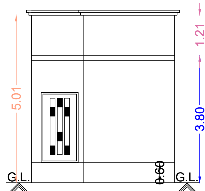
Front Elevation
