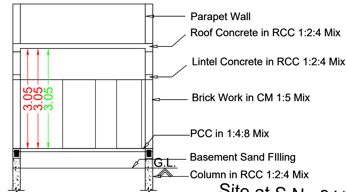
Section RR
