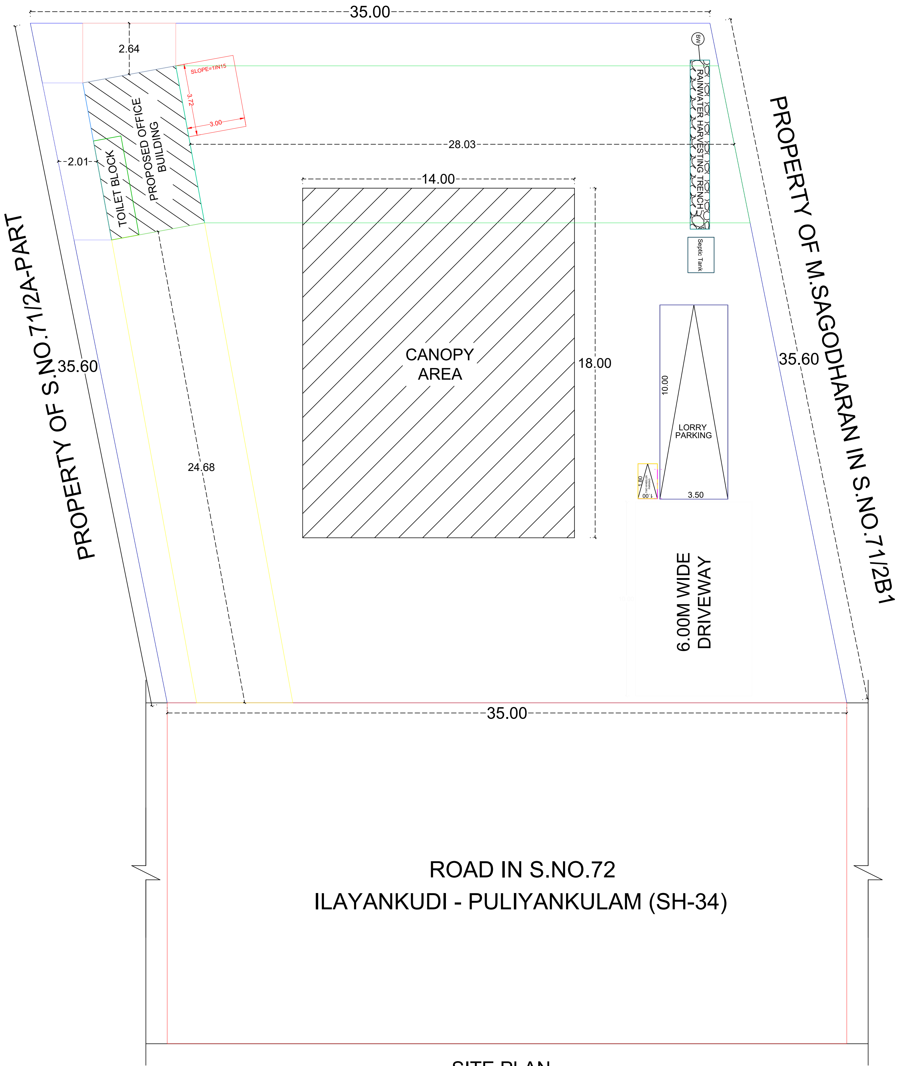
SITE PLAN (1:100)
