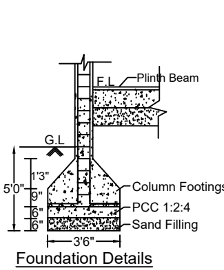
Foundation Details
