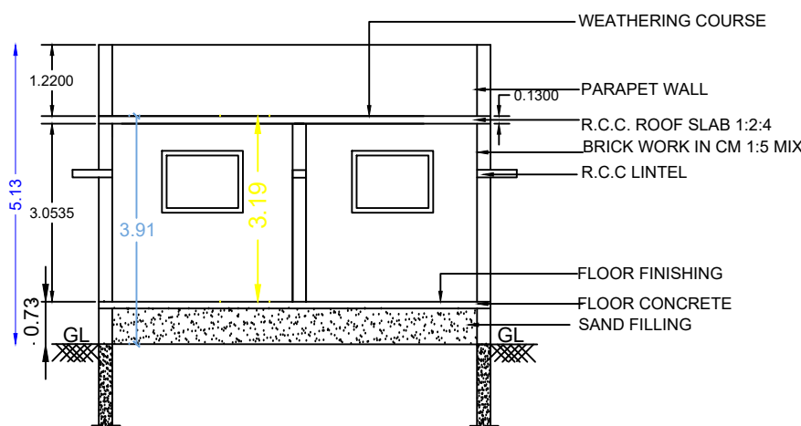
SECTION A1-A1
