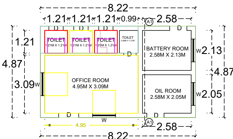
OFFICE & TOILET FLOOR PLAN
