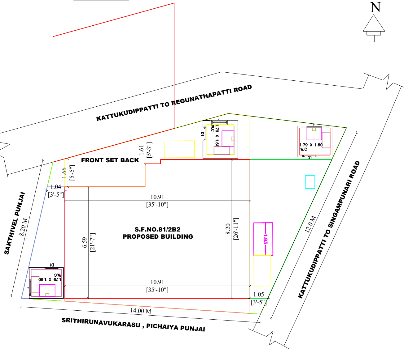
SITE PLAN
