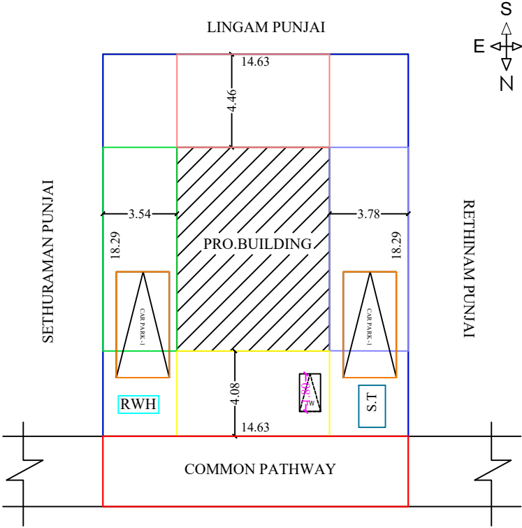
SITE PLAN
