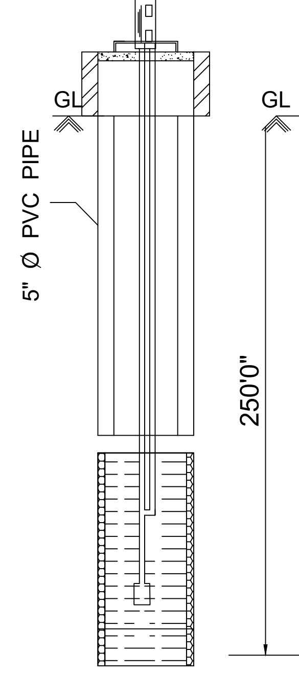
BOREWELL DETAILS
