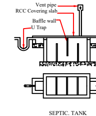
SEPTIC TANK
