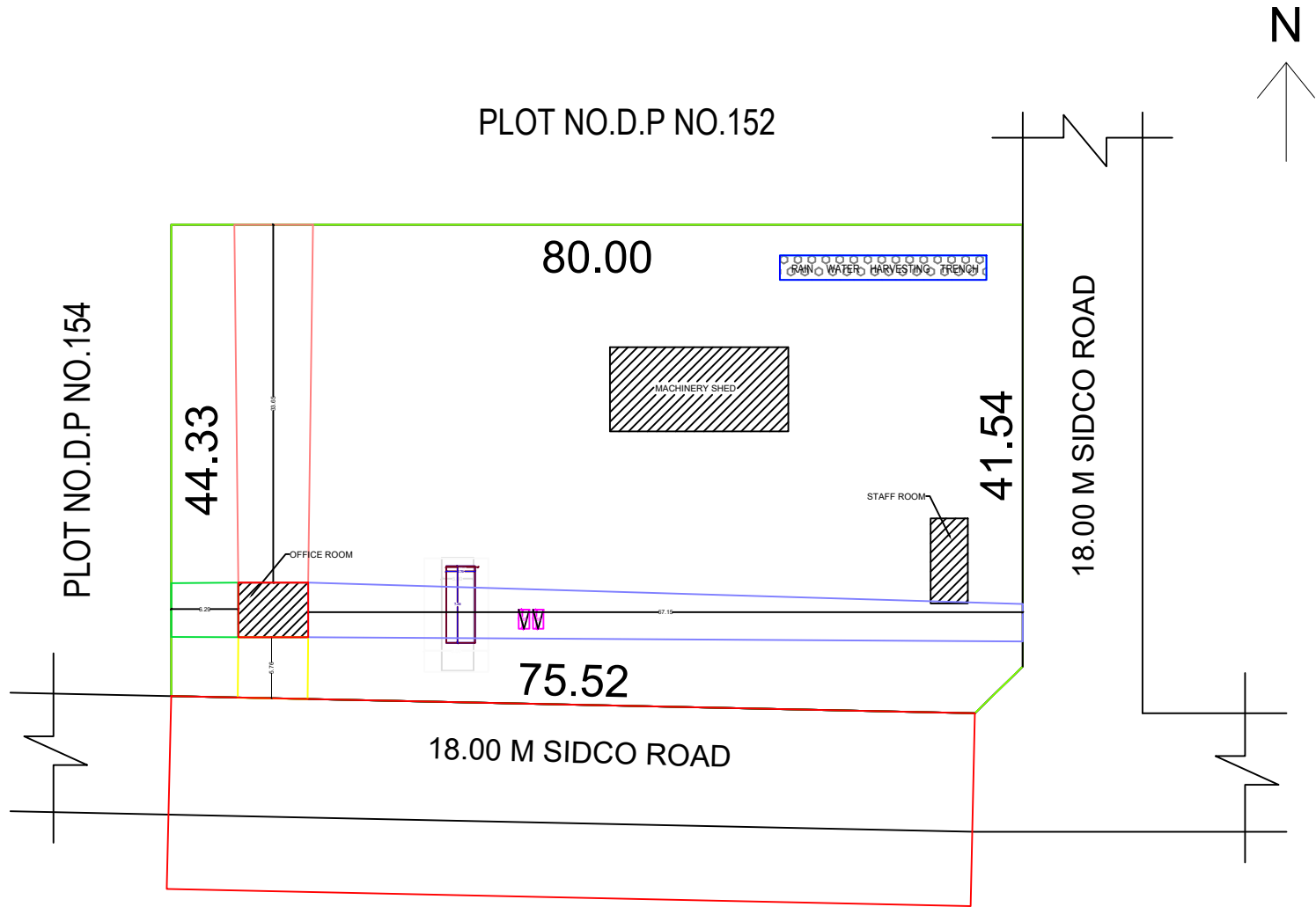
SITE PLAN (SCALE-1:00)
