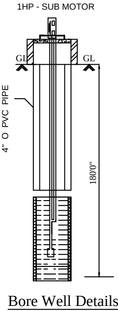
Bore Well Details
