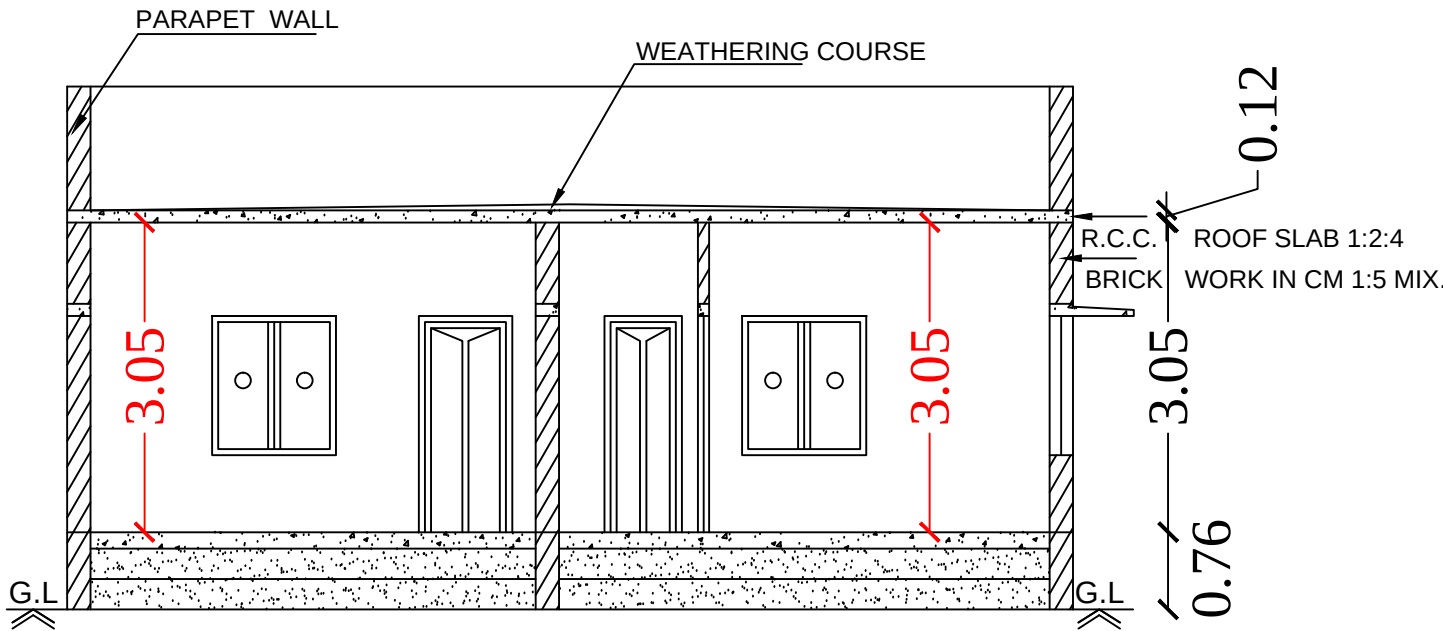
Section on-"AA"
