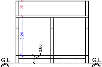
Section on-"AA"
