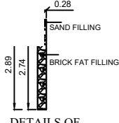
DETAILS OF PERCULATION PIT
