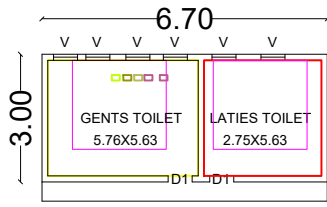
TOILET BLOCK
