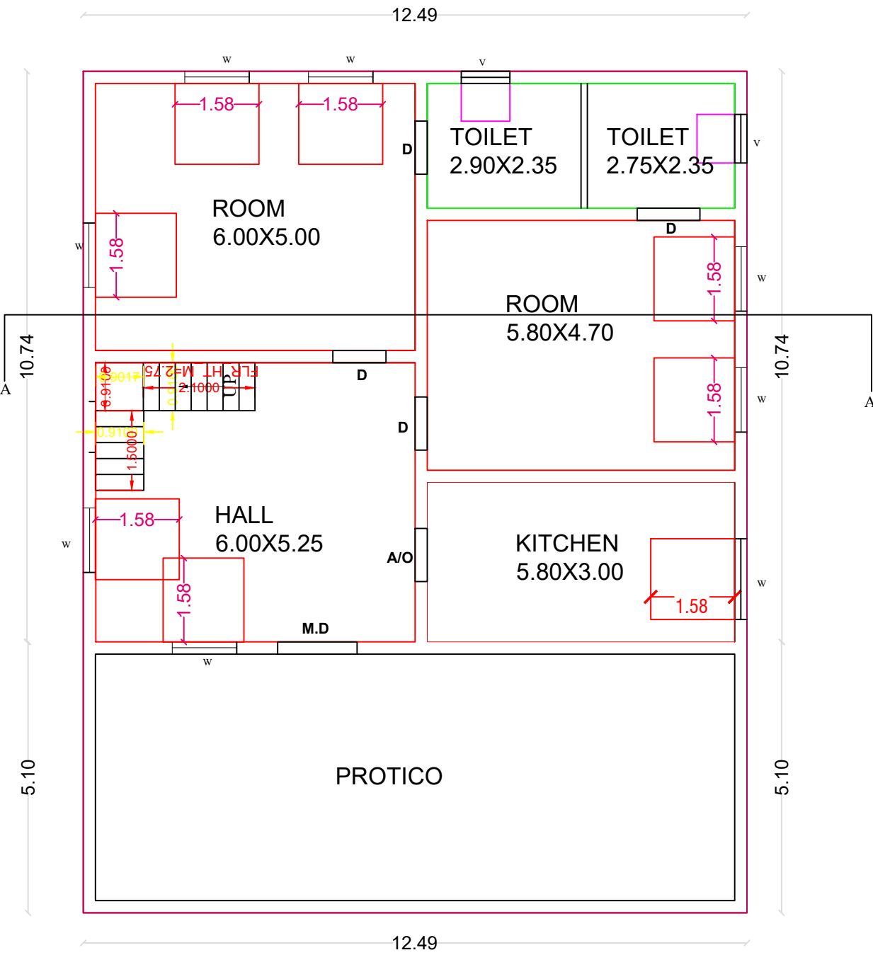
GROUND FLOOR
