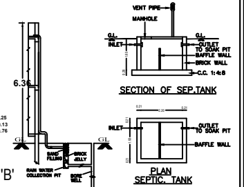
PLAN SEPTIC TANK
