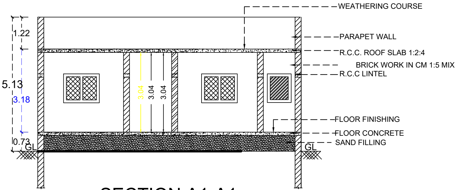
SECTION A1-A1
