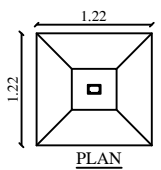
FOUNDATION DETAILS
