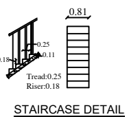
STAIRCASE DETAIL
