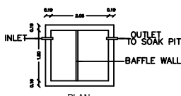
SEPTIC TANK DETAILS
