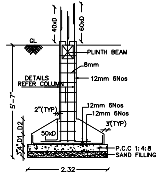
TYPICAL SECTION OF R.C.C. COLUMN FOUNDATION
