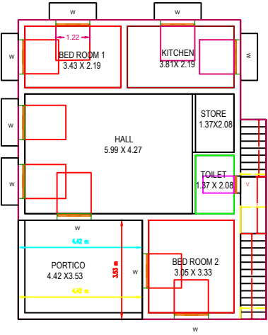
PROPOSED GROUND FLOOR PLAN (DWELLING - 1)
