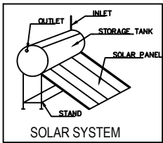
SOLAR SYSTEM
