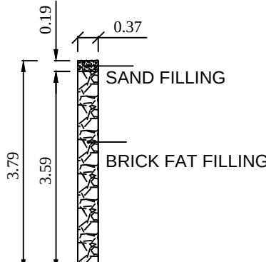
DETAILS OF PERCUSSION PIT
