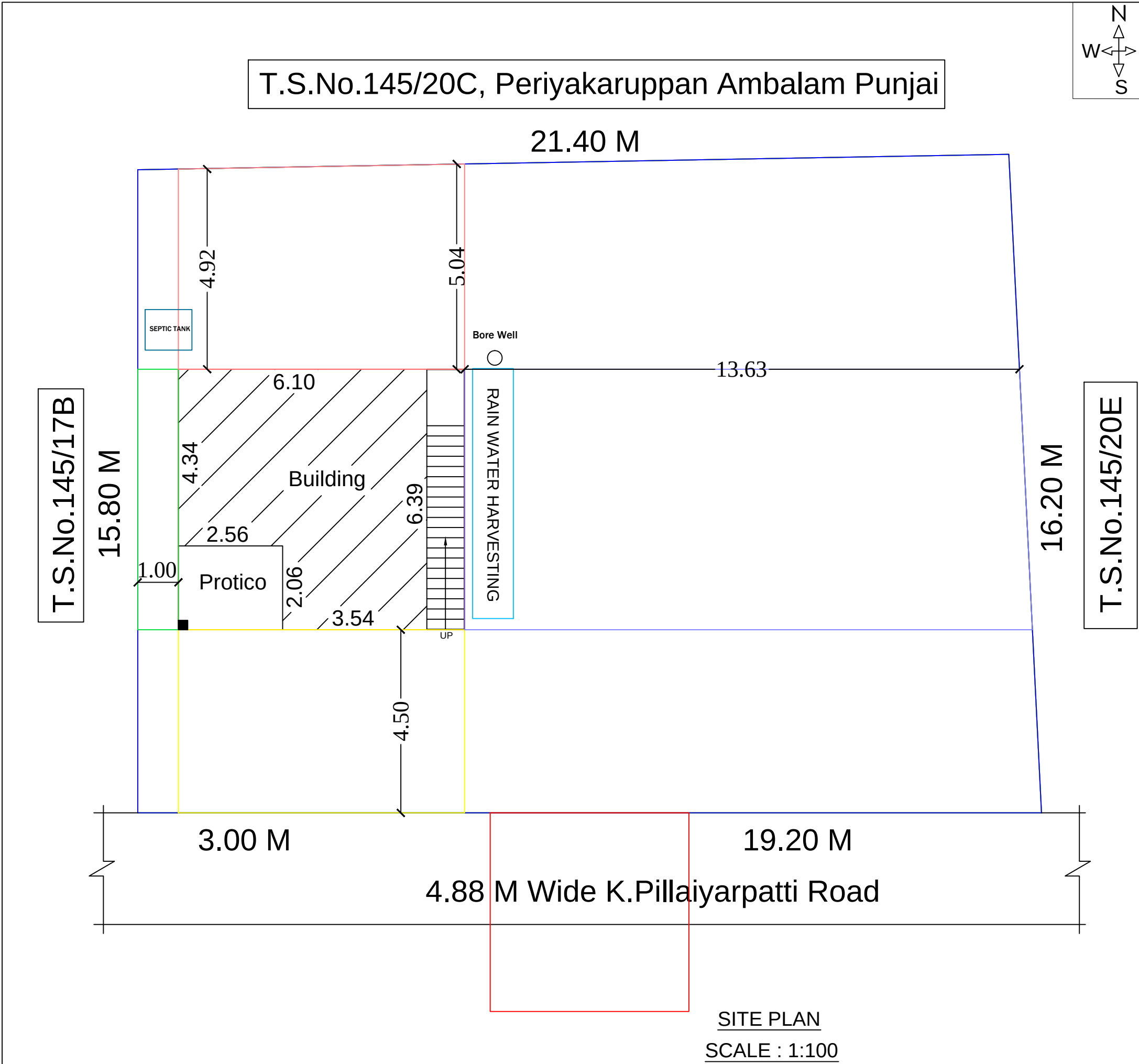
RAIN WATER HARVESTING SYSTEM
