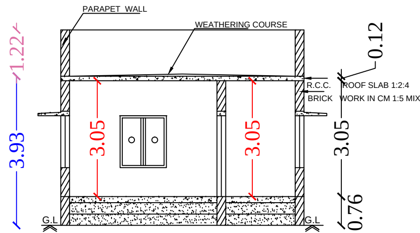
Section on-"AA"
