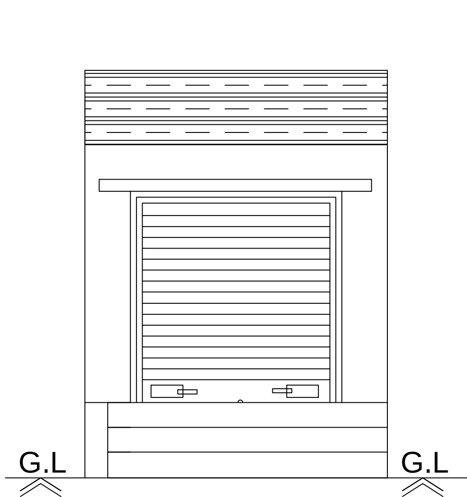
Front Elevation
