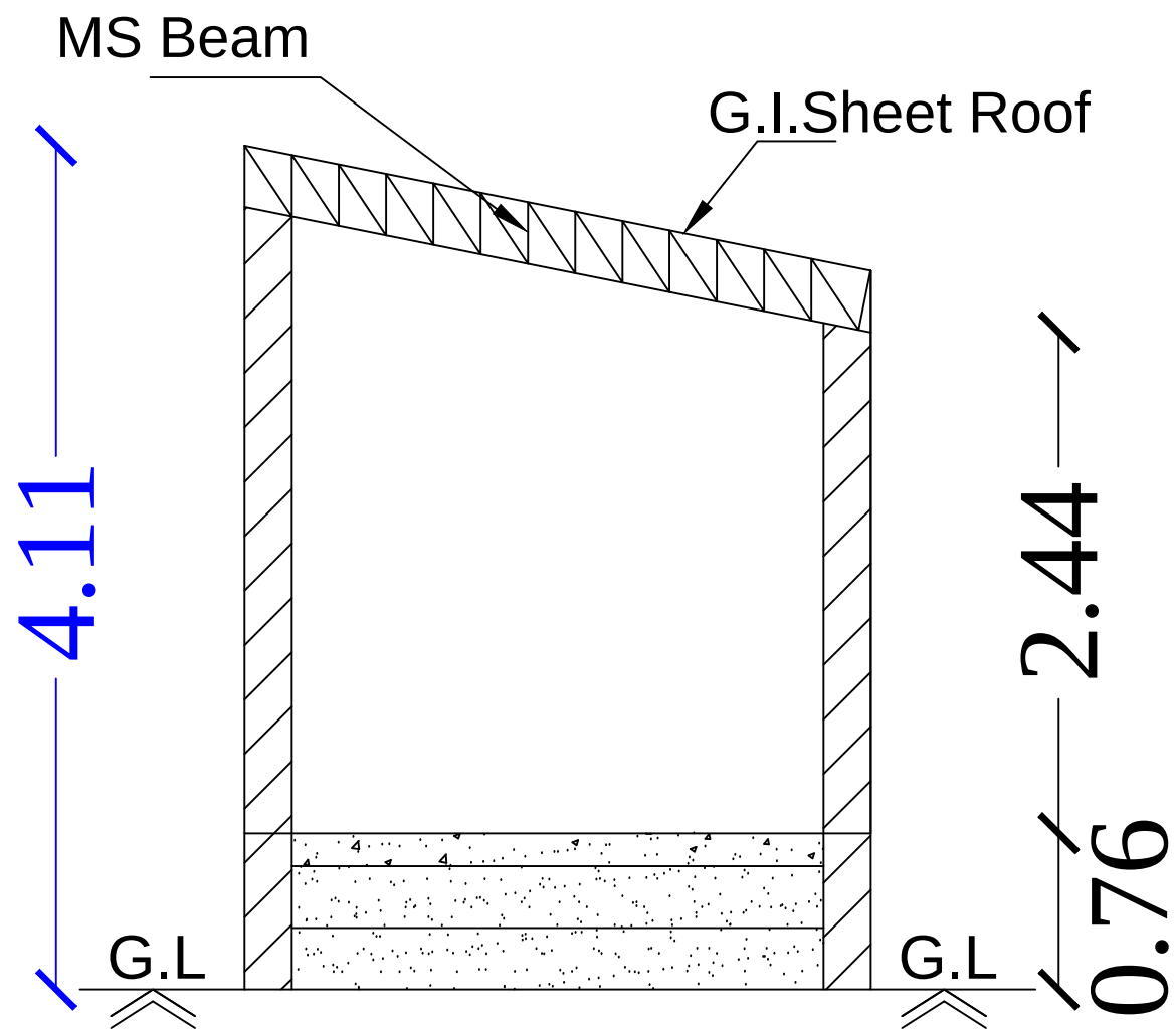
Section on-"AA"
