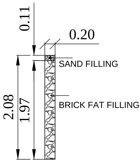
DETAILS OF PERCOLATION PIT
