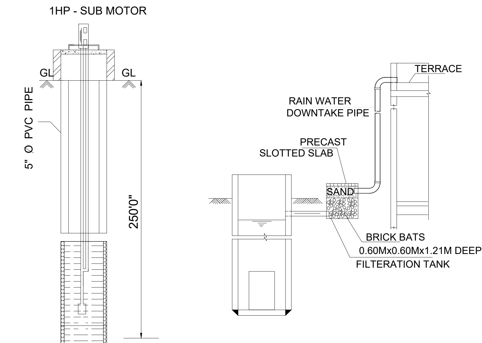
RAIN WATER HARVESTING SYSTEM
