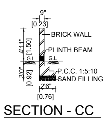
SECTION - CC
