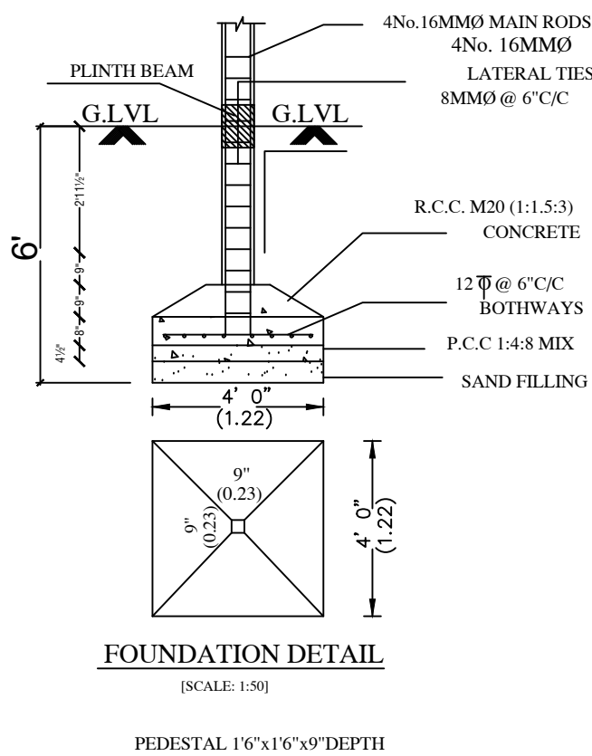
FOUNDATION DETAIL
