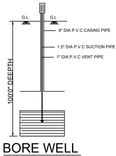
BORE WELL
