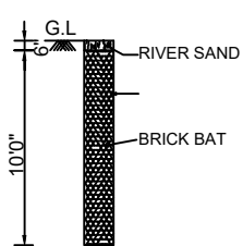
PERCUSSION PIT
