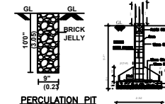
FOUNDATION DETAILS SCALE : 1:50.
