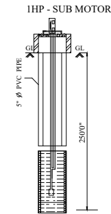
BOREWELL DETAILS
