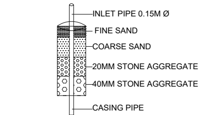
DETAILS OF RAIN WATER HARVESTING STRUCTURES
