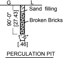
PERCOLATION PIT
