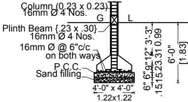
COLUMN DETAILS
