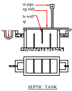
SEPTIC TANK
