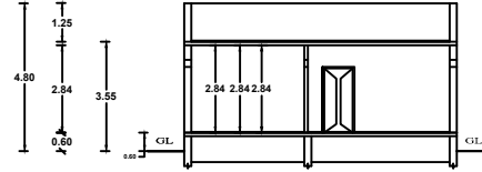
SECTION ON "A B"
