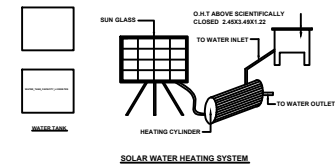
SOLAR WATER HEATING SYSTEM
