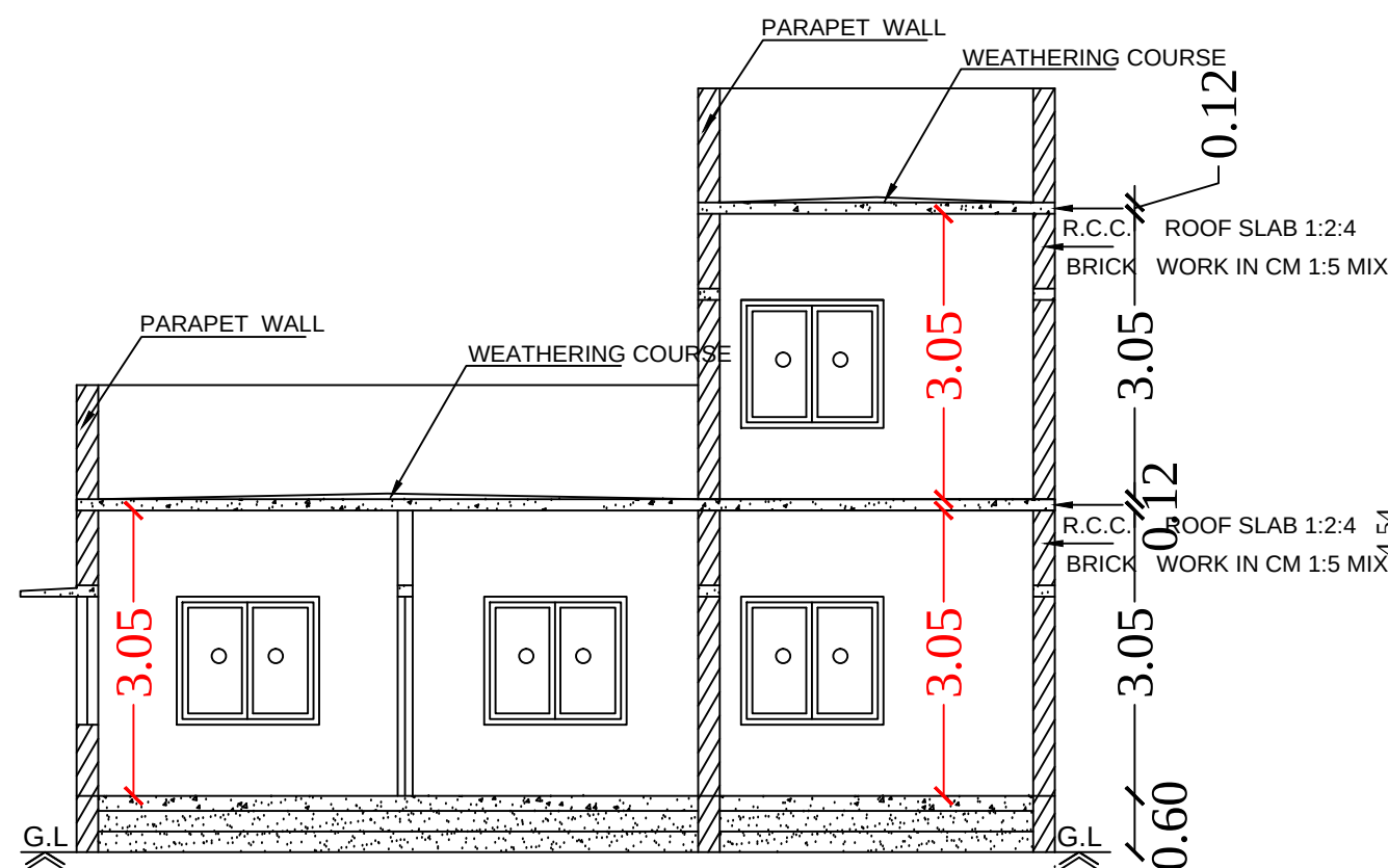
Section on-"AA"
