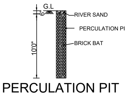
PERCOLATION PIT
