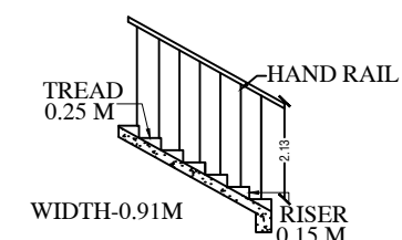
STAIRCASE DETAILS
