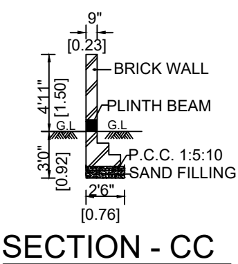
SECTION - CC
