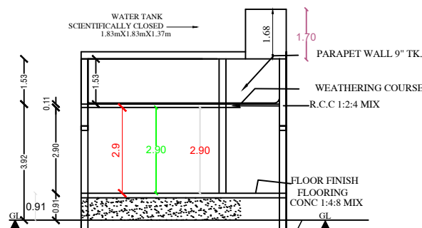
SECTION ON "M-L"
