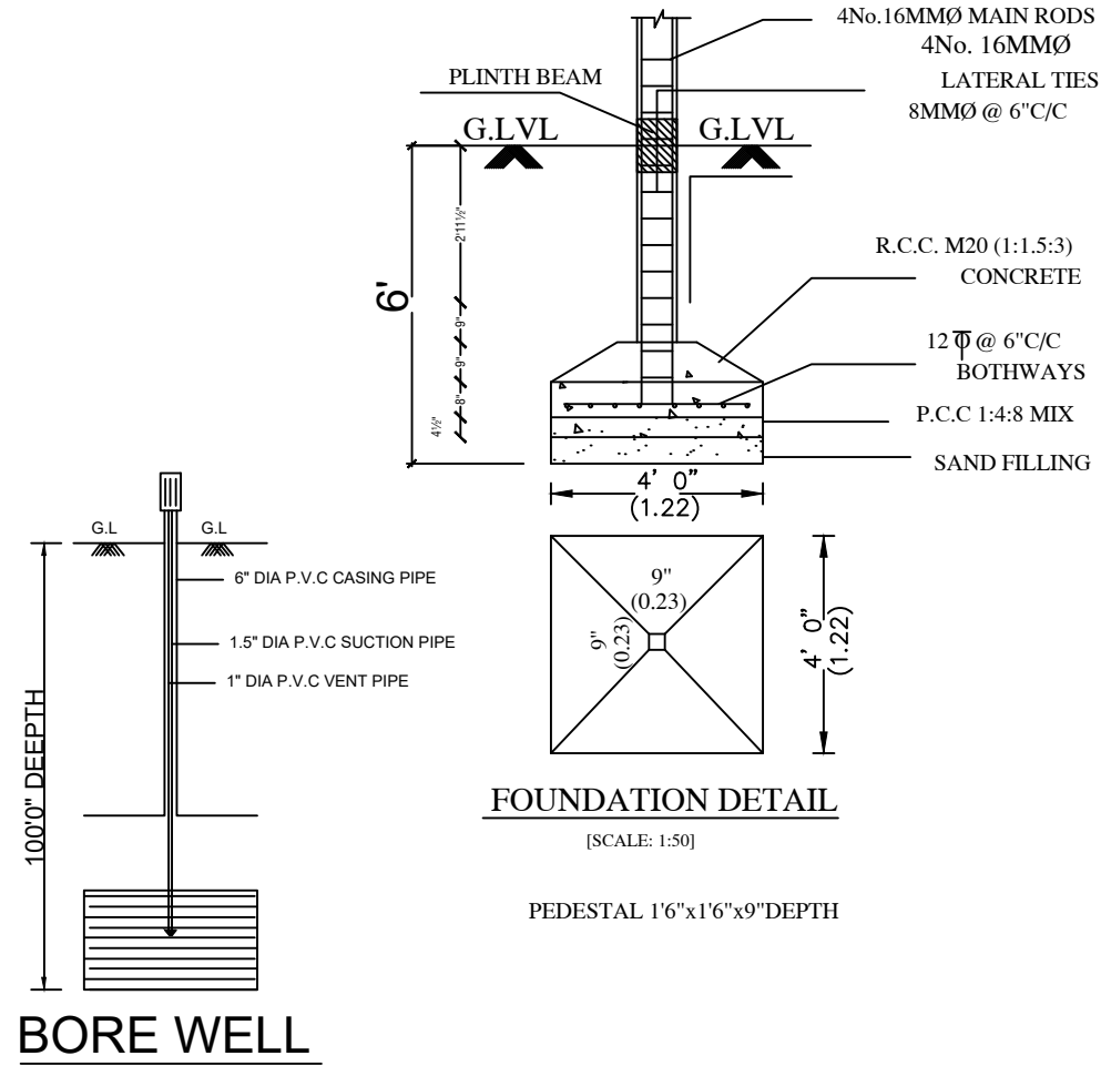
BORE WELL
