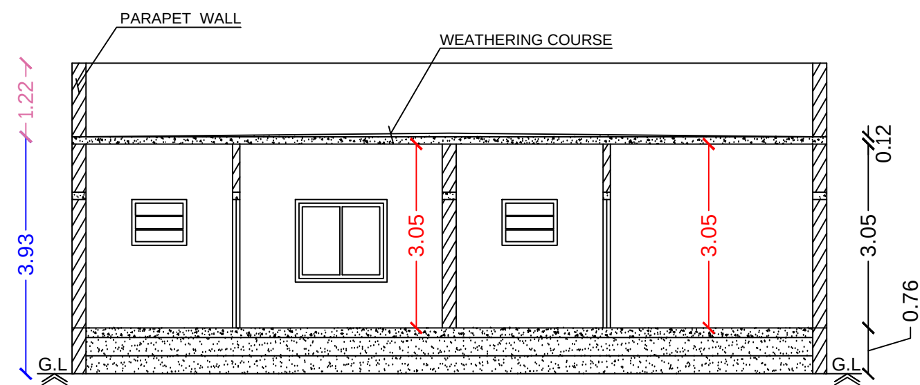
Section on-"AA"
