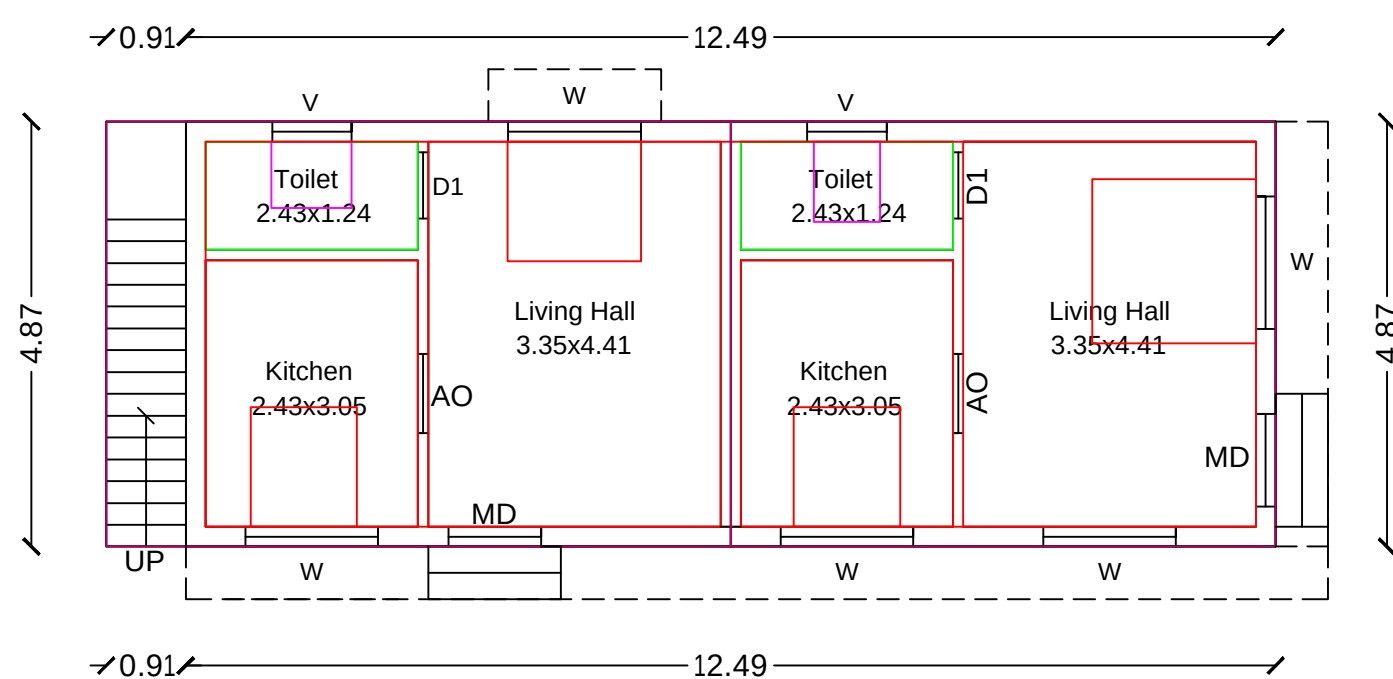
Ground Floor
