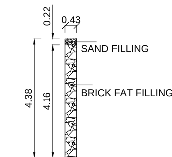
DETAILS OF PERCULATION PIT
