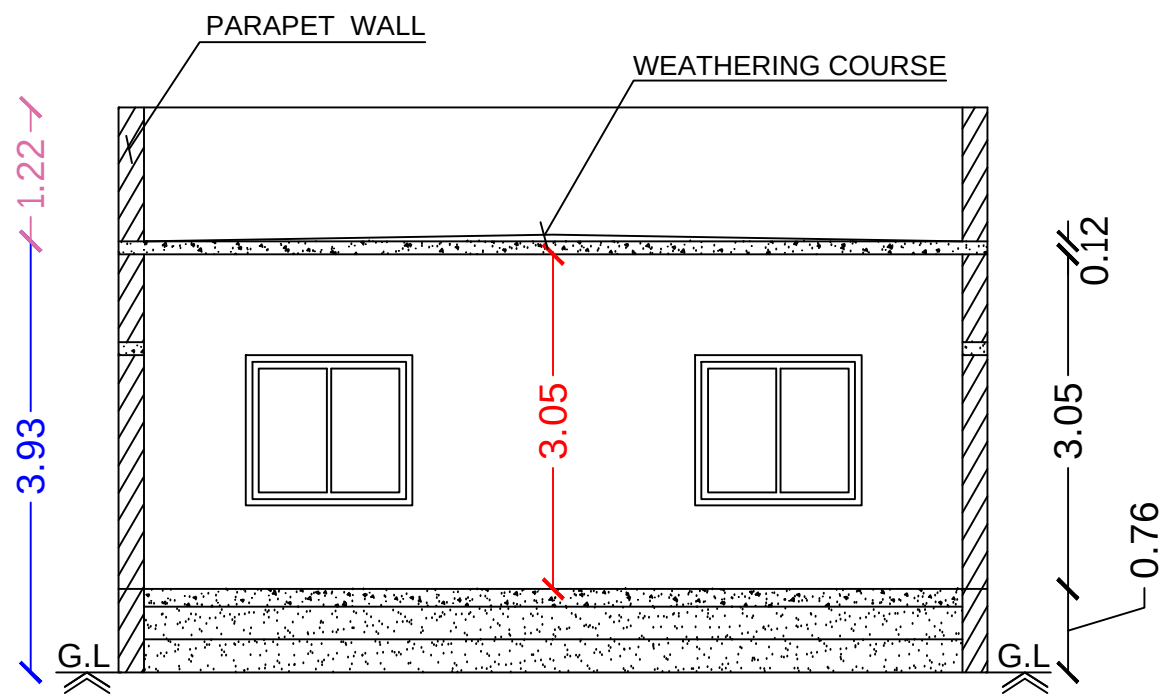
Section on-"AA"
