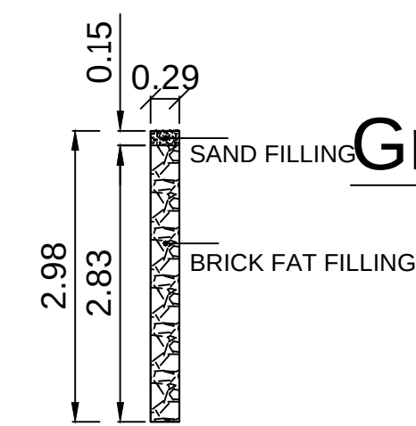
DETAILS OF PERCOLATION PIT
