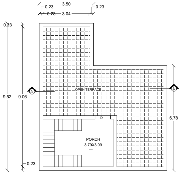
TERRACE FLOOR
