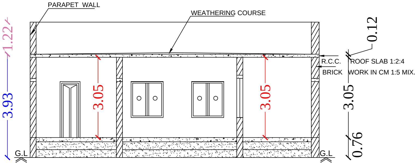
Section on-"AA"
