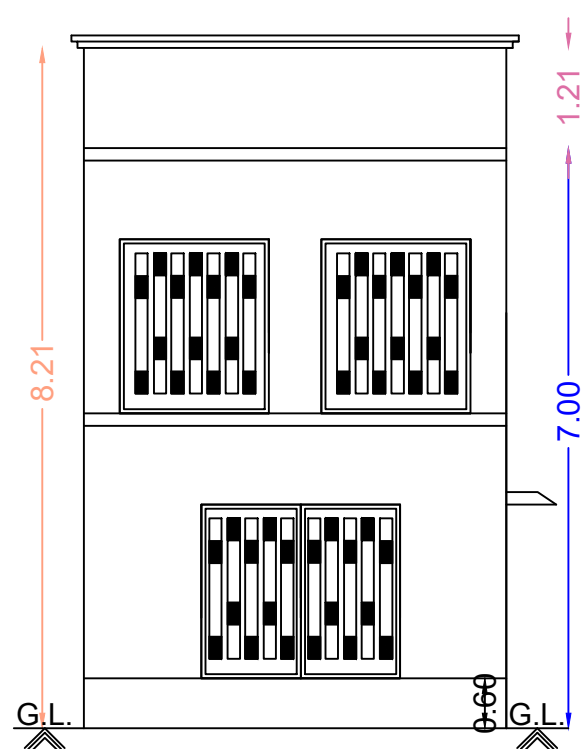
Front Elevation
