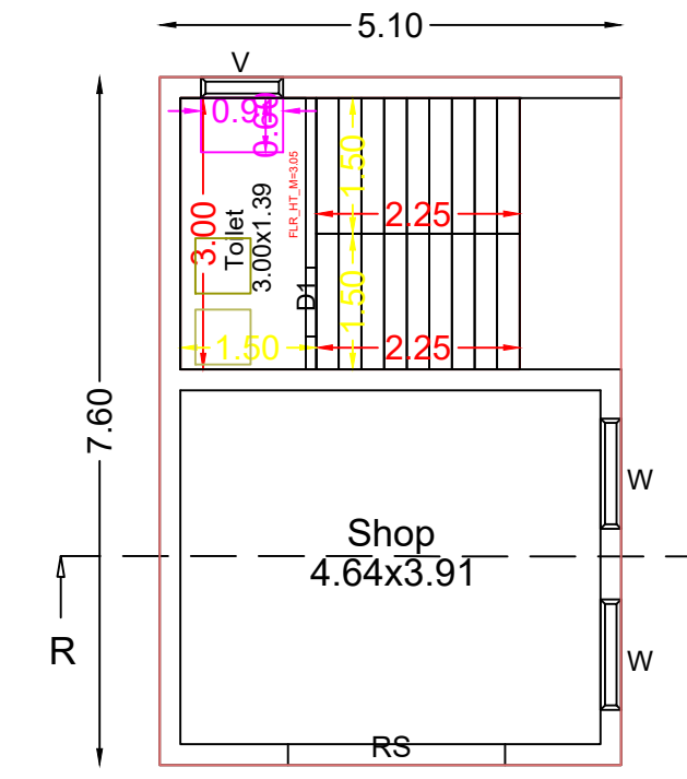
Ex.Ground Floor Plan
