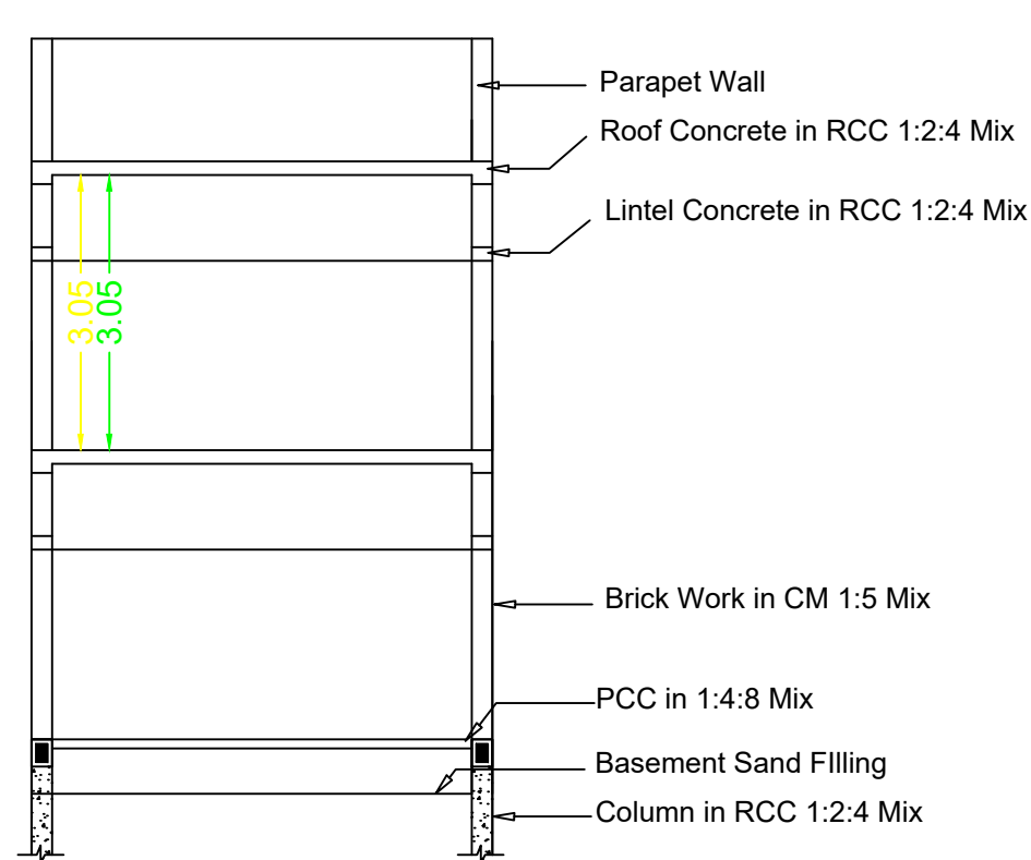
Section RR
