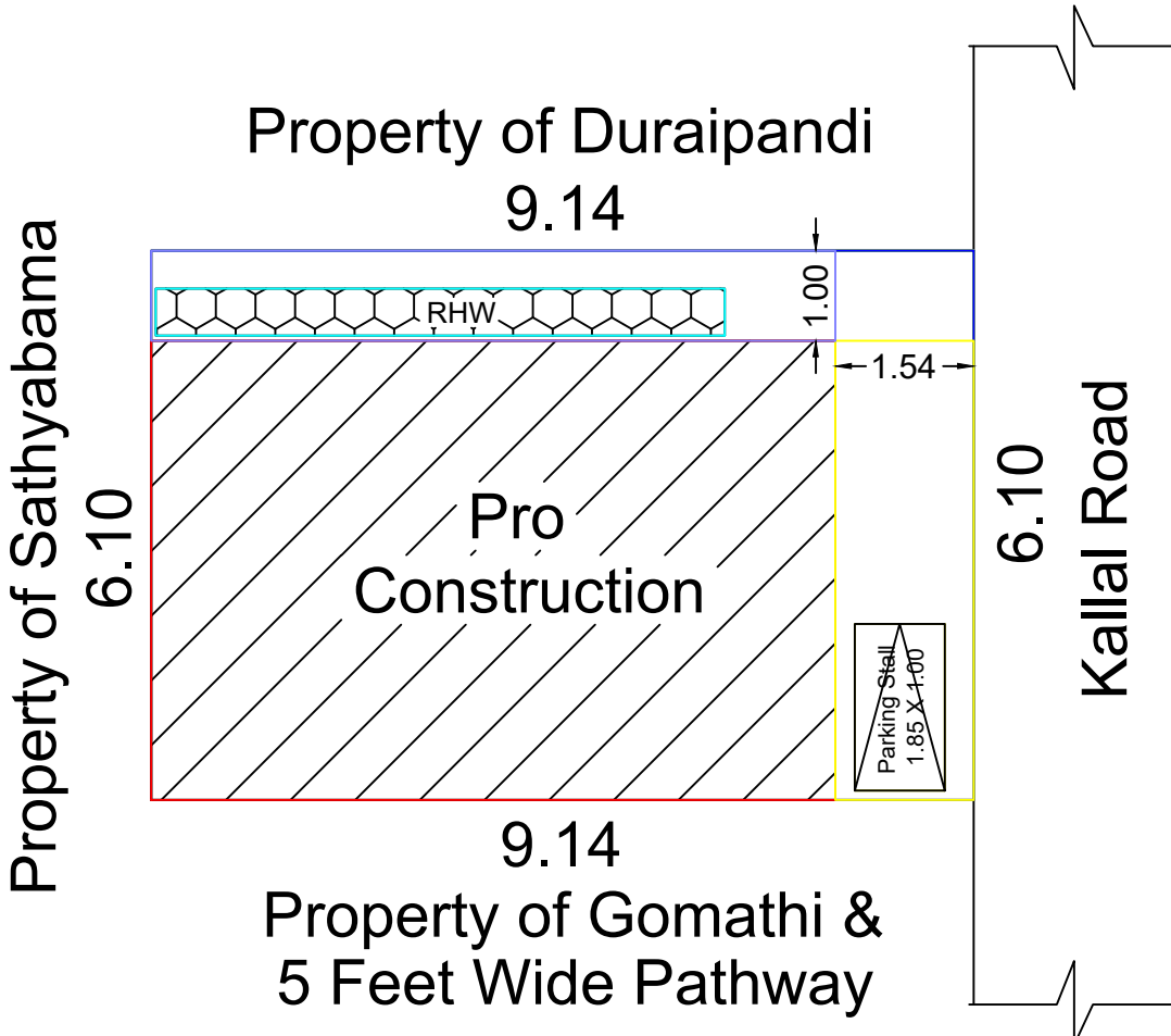
Site Plan
