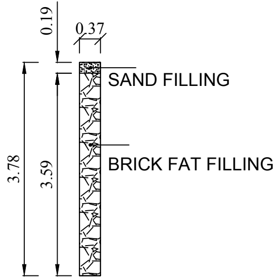
DETAILS OF PERCULATION PIT
