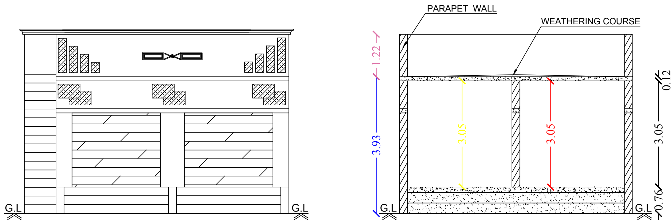
Front Elevation
