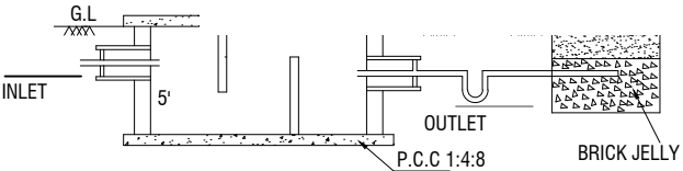
SECTION-AB
