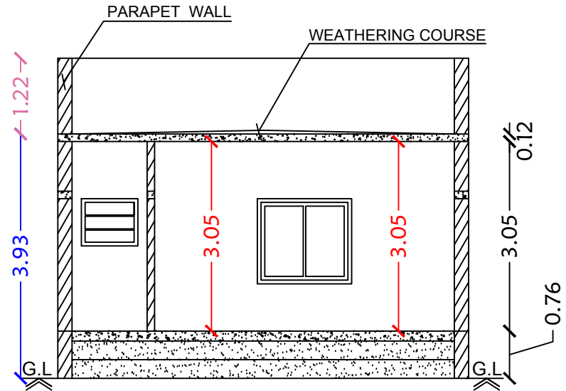
Section on-"AA"
